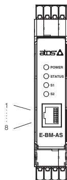
RJ45 connector (IEC 60603 standard) for RS232 serial communication
